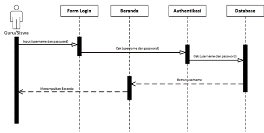
Gambar 6. Sequence Diagram
