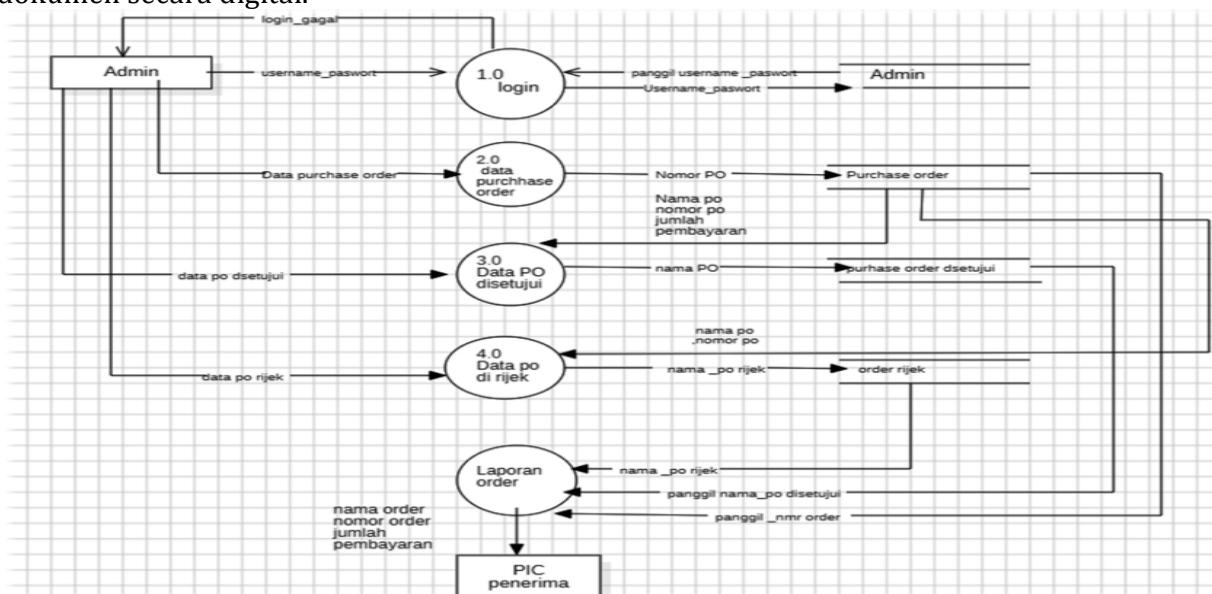
Gambar 3. Diagram Level 1
