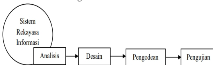
Gambar 1. Metode Waterfall
